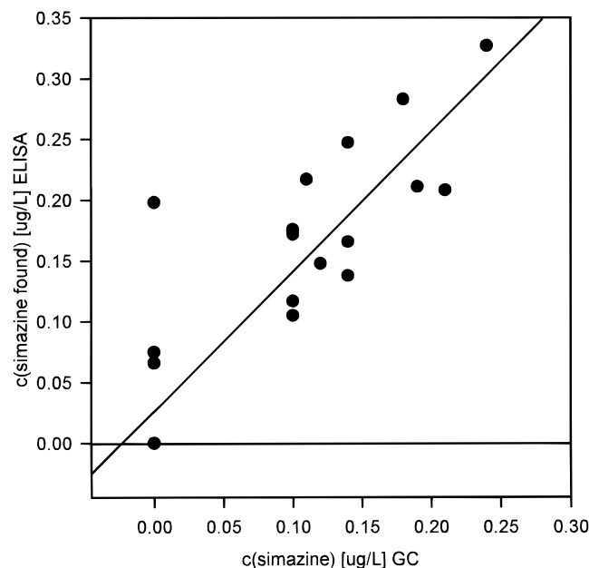
Figure 8. Analysis of ground water samples. Simazine detected by ELISA vs simazine measured by GC. Regression data are R^2 = 0.674 , b = 1.321 , and a = 0.024 (28 points).
