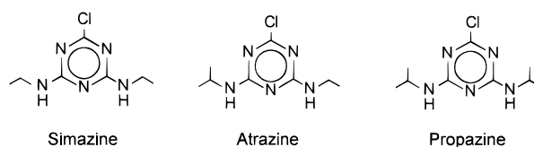
Figure 1. Structures of the three triazine herbicides simazine, atrazine, and propazine.
