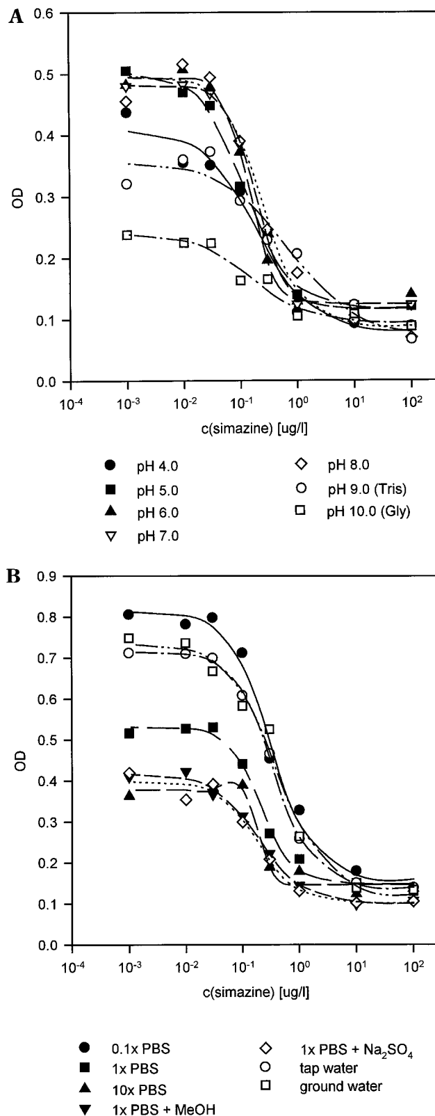
Figure 6. (A) Influence of varying pH on the simazine calibration curve. The ionic strength was constant in all buffers. (B) Influence of the ionic strength on the simazine calibration curve. Low ionic strength results in higher optical density but also in higher IC_{50} .
