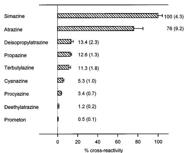
Figure 4. Cross-reactivity pattern of antibody 2282 against a panel of triazine herbicides. The error bars represent the standard deviation calculated from replicate calibration curves which were obtained with the same set of standards ( n = 6 curves for simazine, n = 4 for all others). All other triazines listed in Table 1 showed a cross-reactivity of less than 0.2%.
