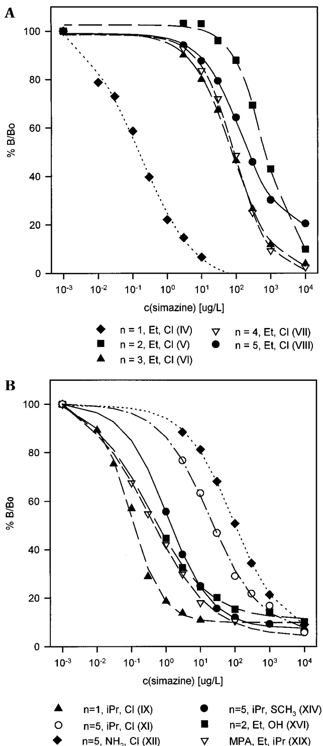
Figure 3. Dose–response curves for simazine using an array of different coating haptens. n = number of carbon atoms in the handle in R^2 ; Et, ethylamino; iPr, isopropylamino; OH, hydroxy; MPA, mercaptopropanoic acid in R^1 . The structure of the hapten largely determines the location of the IC_{50} and therefore the assay sensitivity. Haptens with short spacers (“handles”) generally result in more sensitive assays. No curves were obtained with haptens XIII , XV , XVII , XVIII , and XX . The homologous system III was not tested. Three replicates of each standard were analyzed. The simazine concentrations for each calibration curve were chosen after the approximate location of the IC_{50} was known from previous experiments.
