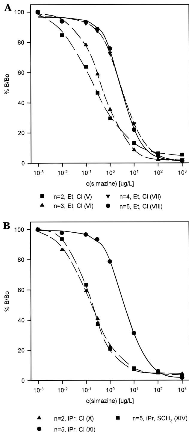
Figure 5. Dose-response curves for simazine using an array of different HRP-hapten tracers. Again, the handle length determines the assay sensitivity. In the tracer format differences in IC_{50} values are less pronounced with the same haptens than in the coating hapten format. No binding was observed to haptens IV and IX . All other haptens not shown have not been investigated. (For abbreviations, see Figure 3.)
