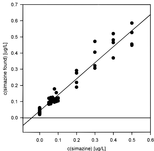
Figure 7. Spike recovery for simazine in tap water at various concentration levels. The regression data for the recovery study are R^2 = 0.943 , b = 0.994 , and a = 0.041 (52 points).
